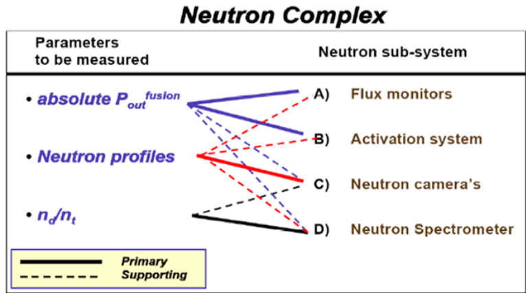
Figure 2. Neutron Complex
